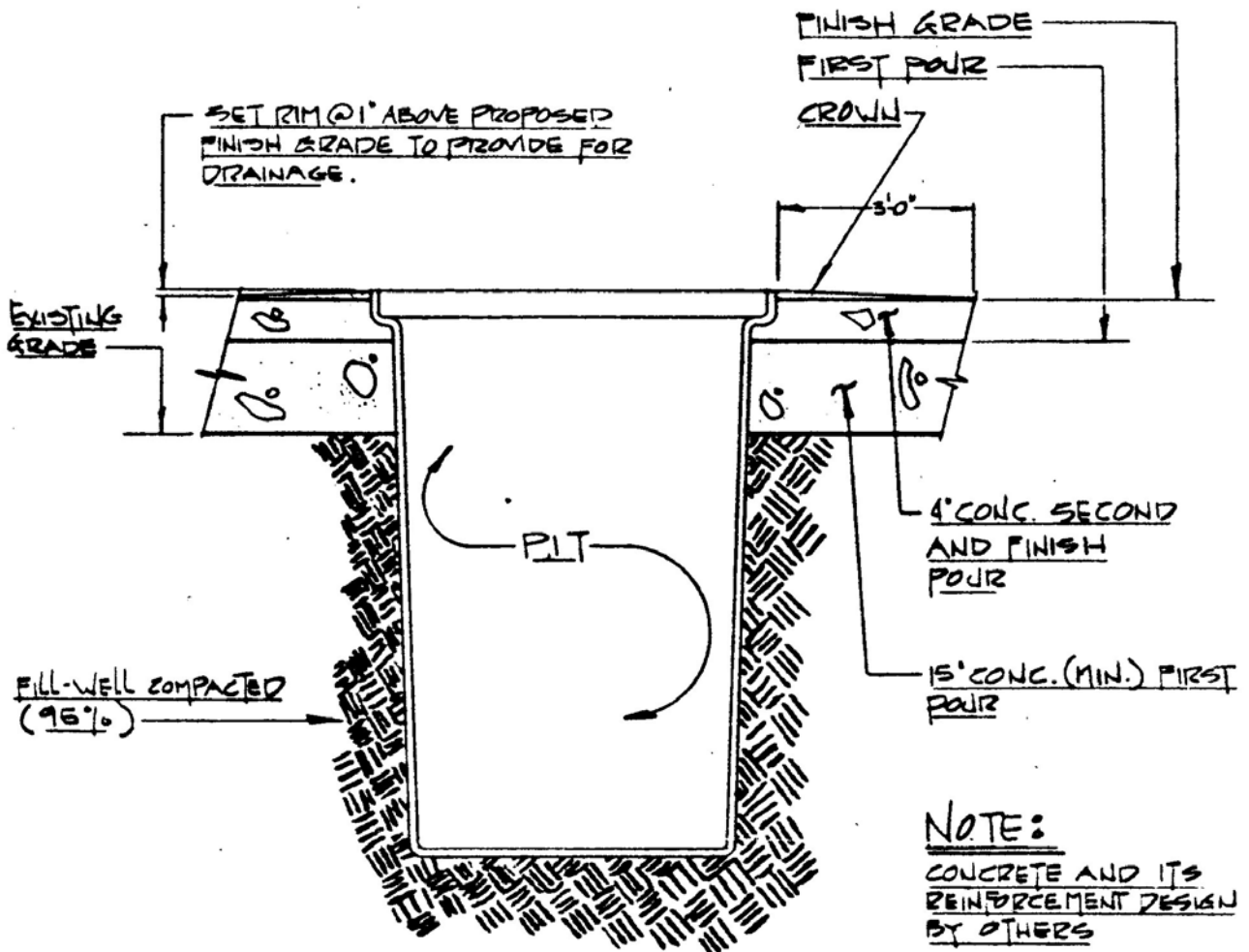
TYPICAL SECTION THRU PIT
