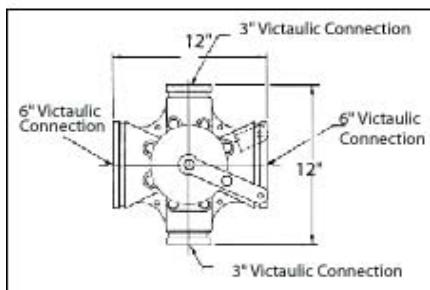
Victaulic porting
