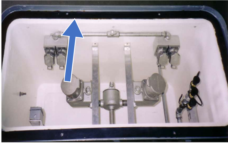
Water Resistant Flat Gasket installed on all four sides of the outer cover (Model 6000WR)
